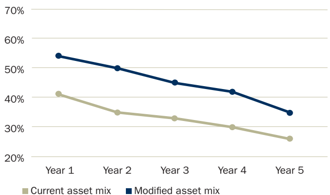
Probability of exceeding $2.5 million annual contribution target
